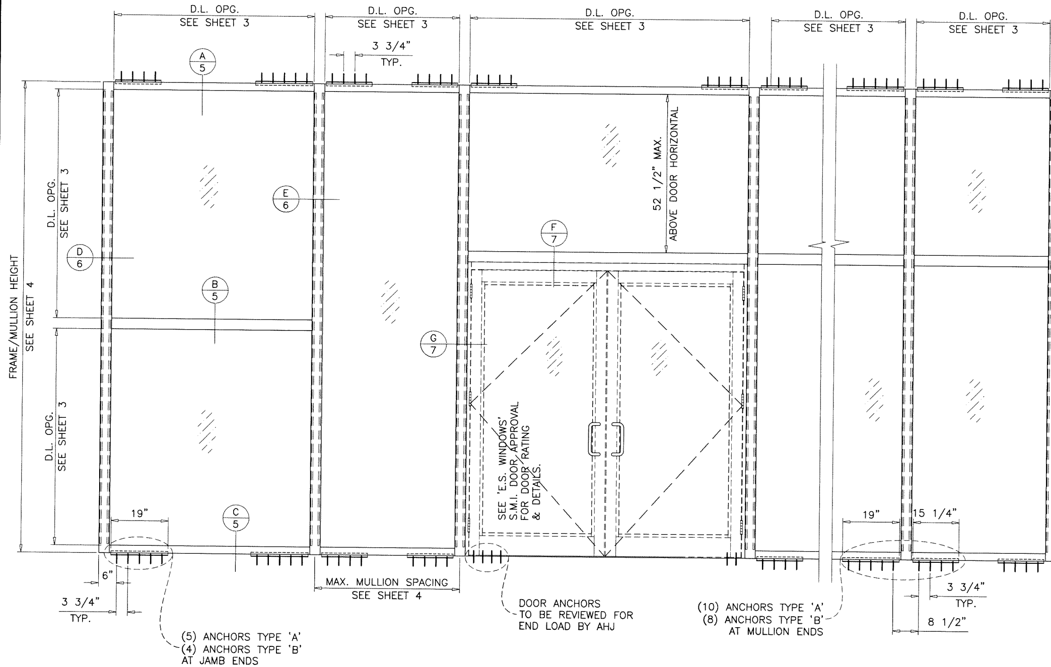
TYPICAL ELEVATIONS
